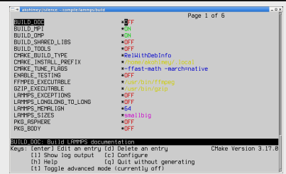
Fig. 6: Options screen of cmake
