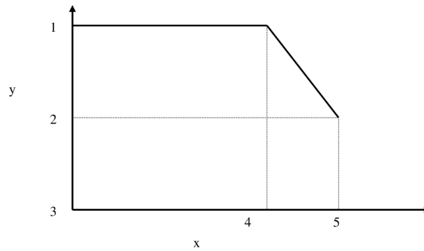
(b) Plot of \nu(\mathbf{x}_p - \mathbf{x}_i) vs. \|\mathbf{x}_p - \mathbf{x}_i\| .
