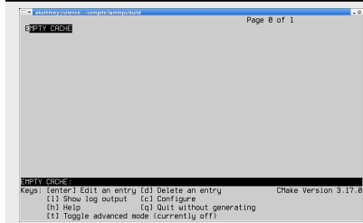
Fig. 4: Initial cmake screen
