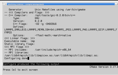
Fig. 5: Configure output of cmake
