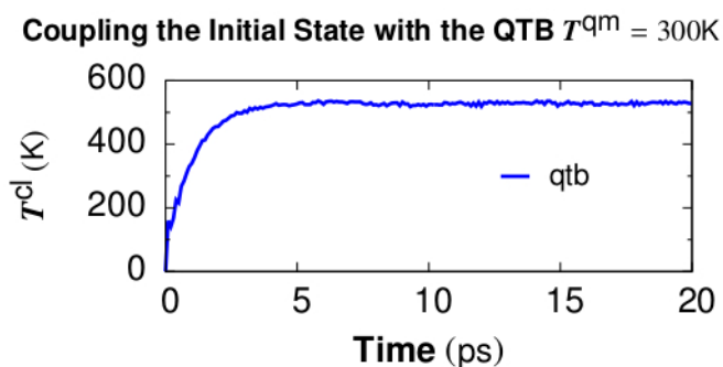
Figure 1. Classical temperature T_{cl} = \sum \frac{mv_i^2}{3Nk_B} vs. time for coupling the \alpha -quartz initial state with the quantum thermal bath at target quantum temperature T^{qm} = 300K . The NpH ensemble is used for time integration while QTB provides the colored random force. T^{cl} converges at the timescale of damp which is set to be 1 ps.
